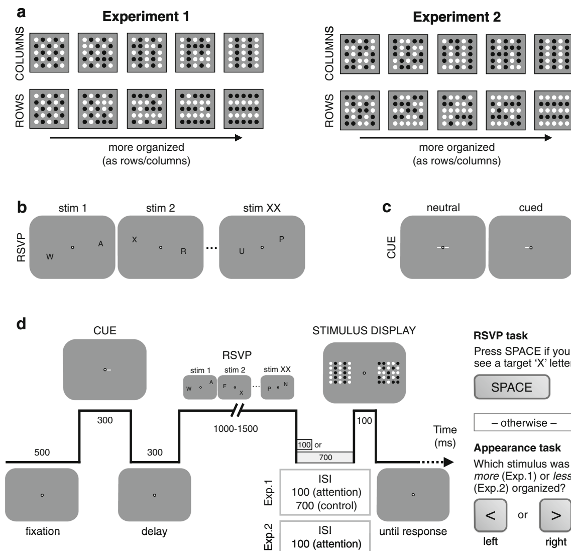
Fig. 1 Experimental procedure. a Perceptual organization stimuli were organized by luminance similarity into columns or rows. The organization level could go from being disorganized in terms of row/column (Experiment 1: checkerboard; Experiment 2: random organization) to a fully organized stimulus. b RSVP sequences were made of a series of letters presented randomly at one of 25 possible locations (5 × 5 grid). c Attention cues were central cues indicating with 100% validity either one (cued) or both (neutral) RSVP streams to attend to.
